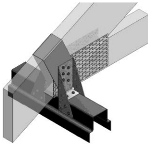
Cyclonic Grip
