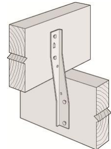
Joist Strap
