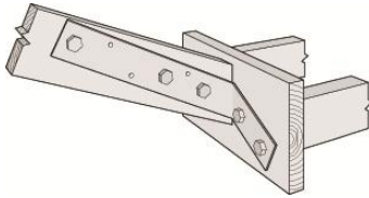
Fascia Support
